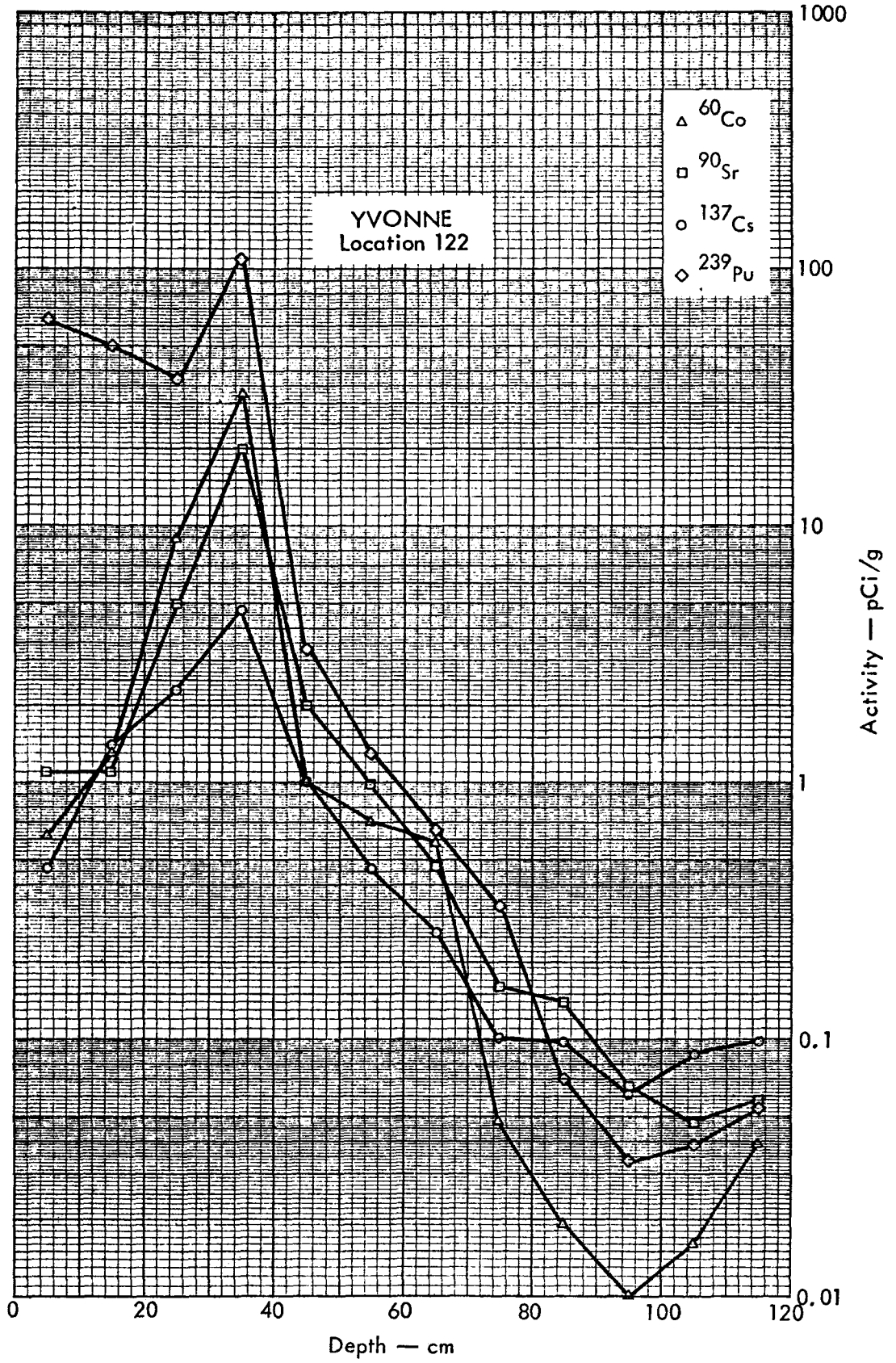
FIGURE 101. ACTIVITIES OF SELECTED RADIONUCLIDES AS A FUNCTION OF SOIL DEPTH
